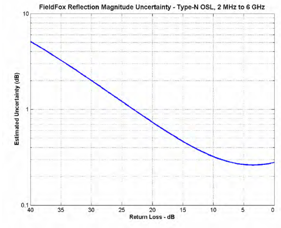
Figure 1: CAT Mode, Type-N Calibration Kit – Magnitude (Specification)
